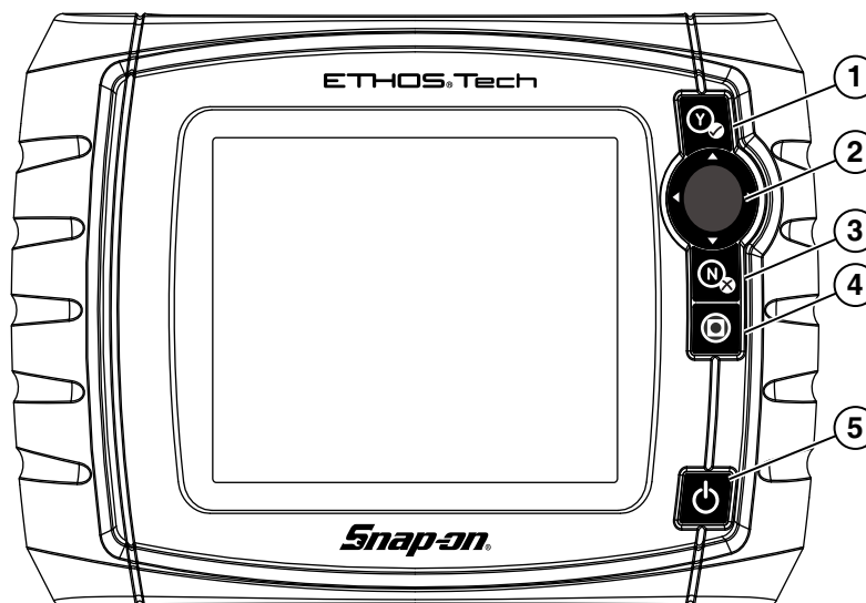
Figure 2-1 Front view
