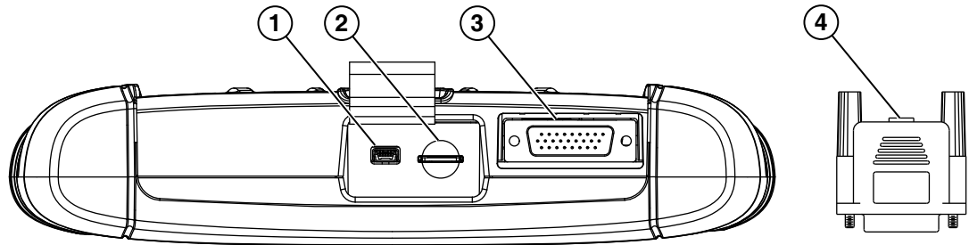
Figure 2-2 Top view
