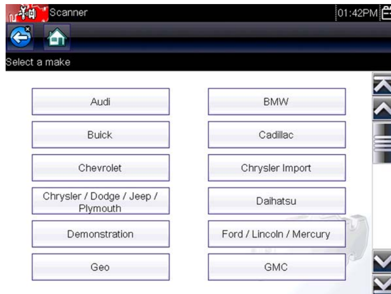
Figure 4-2 Manufacturer list
