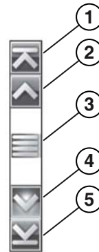
Figure 3-4 Scroll bar
