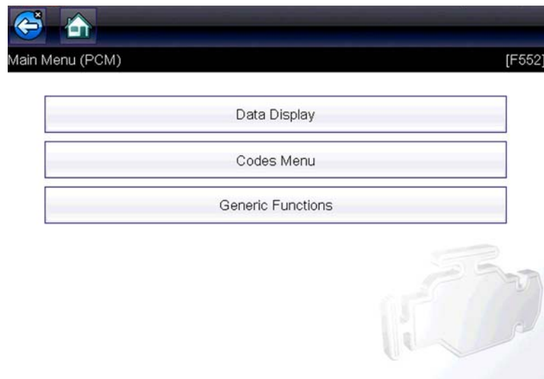
Figure 4-5 Main menu
