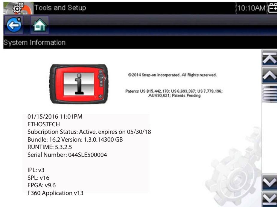
Figure 7-3 System information
