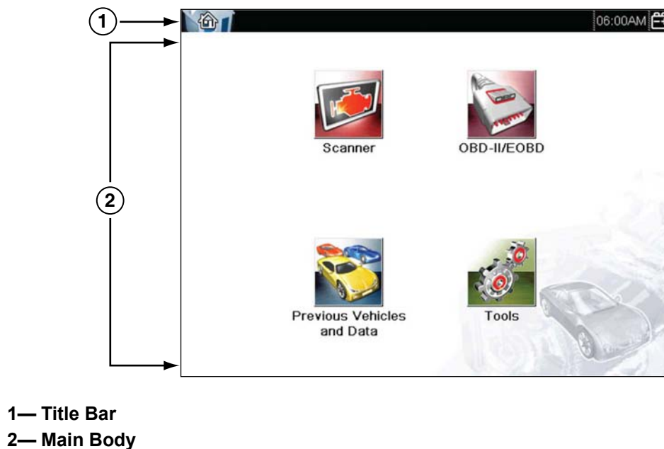
Figure 3-3 Home screen
