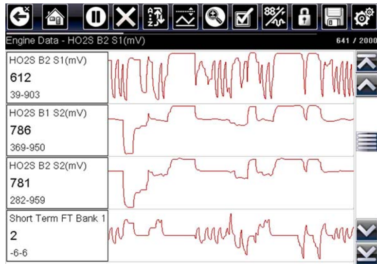
Figure 7-6 High-contrast toolbar
